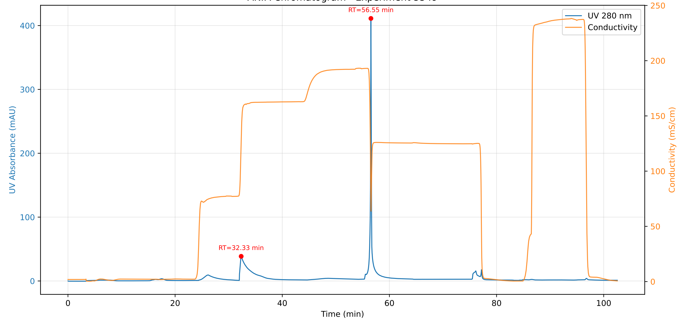
AKTA Chromatogram - Experiment 5549
